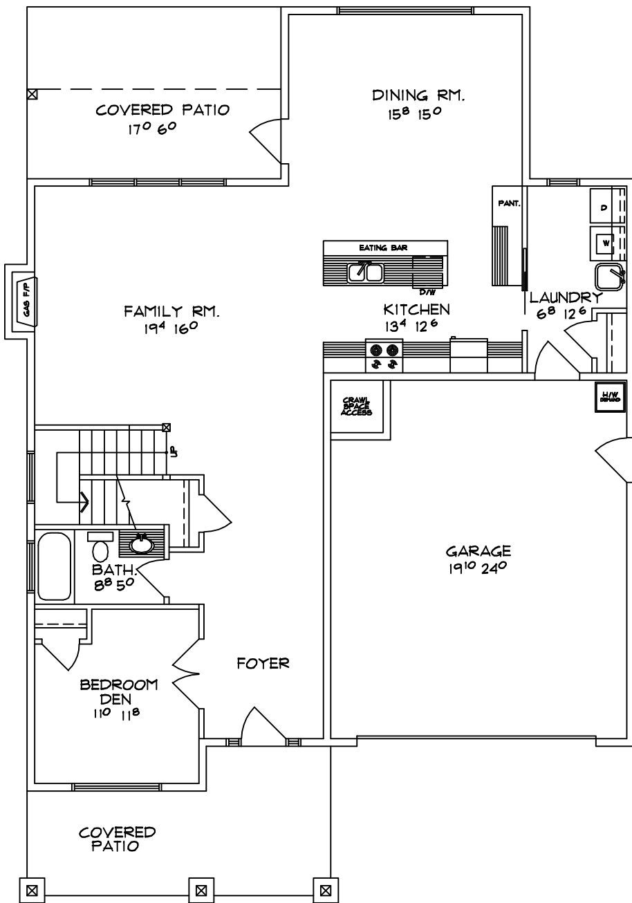
MAIN FLOOR PLAN 1283 SQ. FT.
